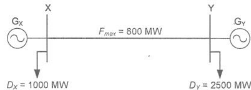
Figure Q6 A simple two-bus power system
